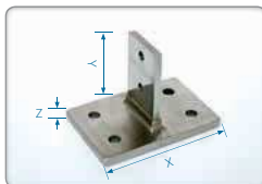
Bodenplatte 120 x 80mm Plaque de base 120 x 80mm
